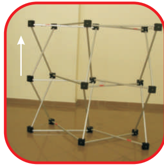
2. Build up construction (A) that plugs for table top were on top. Follow stickers with row "This side Up".
